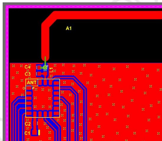
Figure 3.2: Use the external antenna
